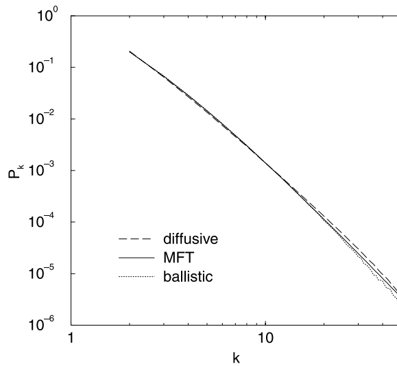
Figure 7. The final distribution of passive clusters for the p = \frac{1}{2} stochastic aggregation with diffusive and ballistic transport. Also shown is the mean-field distribution P_k(\infty) = 24/[k(k+1)(k+2)(k+3)] .
