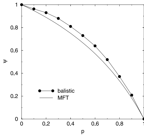
Figure 6. The scaling exponent \psi(p) versus p for ballistic aggregation compared with the mean-field value of equation (8).
