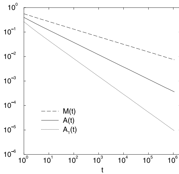
Figure 1. The number density, mass density and monomer density versus time for p = \frac{1}{2} .
