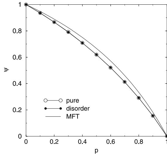
Figure 3. The exponent \psi versus p . Monte Carlo simulation results for the pure diffusion case are compared with the mean-field theory (8) and the exact value for the disordered case. The latter is obtained from U(-2/(2-p), 2\psi, 2) = 0 [7], where U(a, b, z) is the confluent hypergeometric function.
