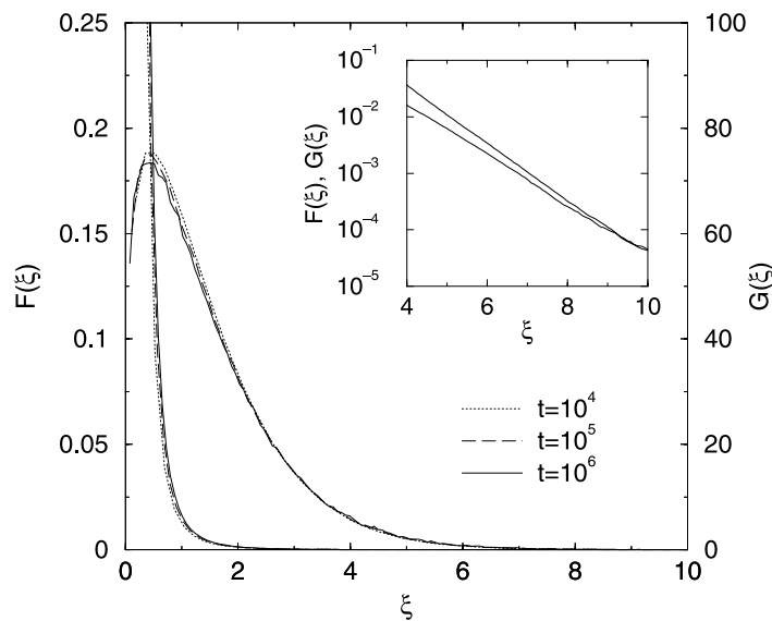
Figure 2. Scaling of the active and passive mass distributions. Shown are the scaling functions F(\xi) \equiv t^{\nu(2-\psi)} A_k(t) and G(\xi) \equiv t^{\nu(2-\psi)} P_k(t) , versus the scaling variable \xi = kt^{\nu(1-\psi)} at three different times t = 10^4, 10^5 and 10^6 . Different scales correspond to F(\xi) and G(\xi) in the main figure since the latter diverges at the origin. The data represent an average over 10^3 independent realizations in a system of size L = 10^6 for the case p = \frac{1}{2} . The exponent value \psi = 0.619 was used. The tail of the distribution is shown in the inset.
