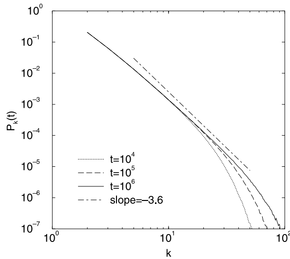
Figure 5. The distribution P_k(t) versus k for three different times t = 10^4 , 10^5 and 10^6 . The typical mass at these three times is proportional to k^* \equiv t^{\nu/(1-\psi)} \propto 6 , 10 and 16 , respectively. Hence, the distribution is fully developed only over a short range of masses. The data represent an average over 10^3 realizations in a system of size L = 10^6 with p = \frac{1}{2} .
