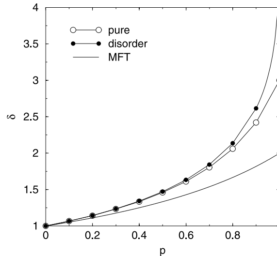
Figure 4. The exponent \delta versus p . Monte Carlo simulation results for the pure diffusion case are compared with the mean-field theory (8) and the exact value for the disordered case obtained from U(-2(1-p)/(2-p), 2\delta, 2) = 0 [7].
